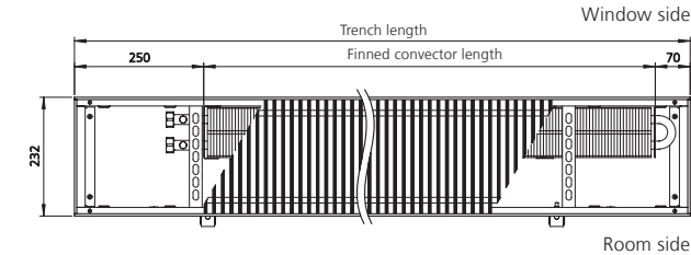
Top view of trench height 92/120 mm (view without cover panel)
