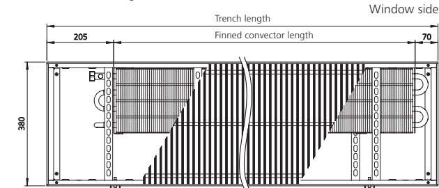
Top view of trench height 150/200 mm (view without cover panel)
