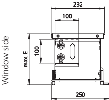
Cross-section through trench height 150/200 mm (example shown with roll-up grille)
