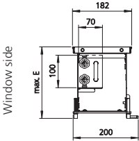
Cross-section through trench height 150/200 mm (example shown with roll-up grille)
