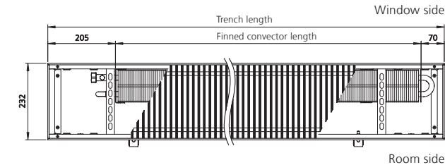
Top view of trench height 150/200 mm (view without cover panel)
