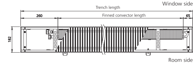
Top view of trench height 92/120 mm (view without cover panel)
