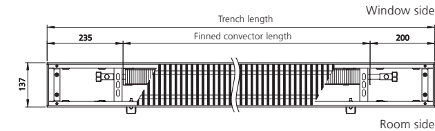
Top view (view without cover panel)
