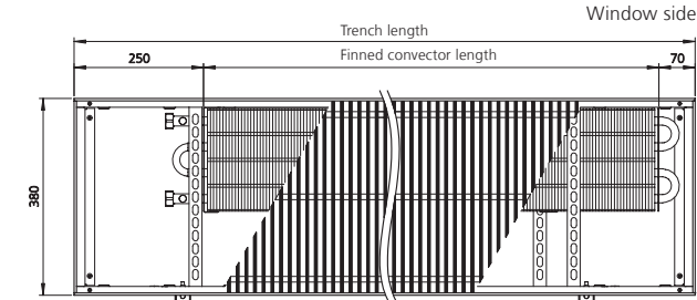
Top view of trench height 92/120 mm (view without cover panel)
