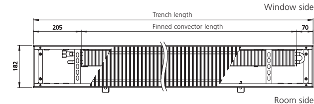
Top view of trench height 150/200 mm (view without cover panel)
